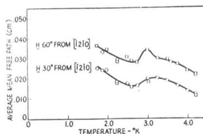
Fig. 1. The electronic mean free path in cadmium sample A as a function of temperature for two different magnetic field directions. The sound direction q is along [10\bar{1}0] .
